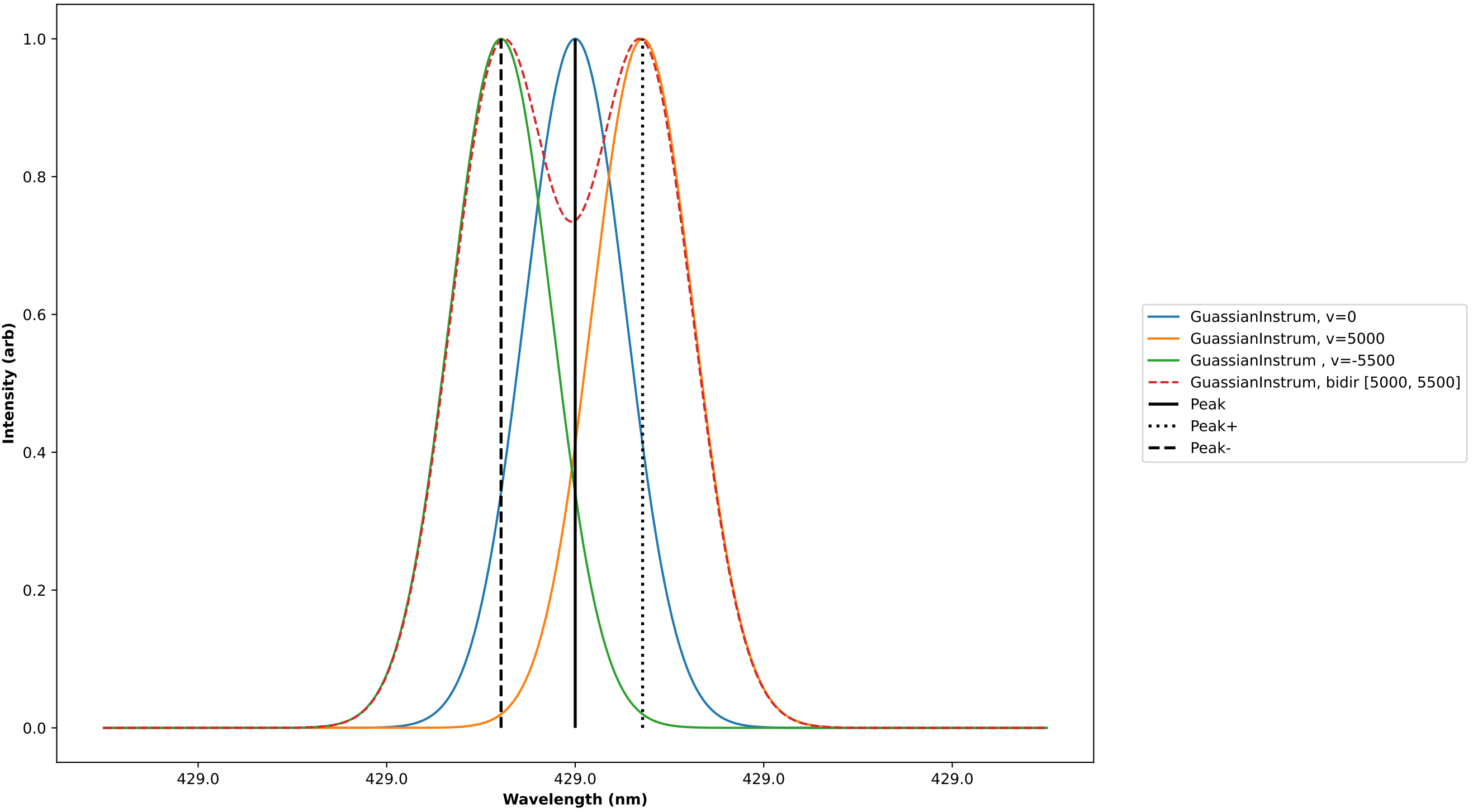
GaussianInstrum: T=10.0 eV, AMU = 183, Pixels = 0.01 nm
